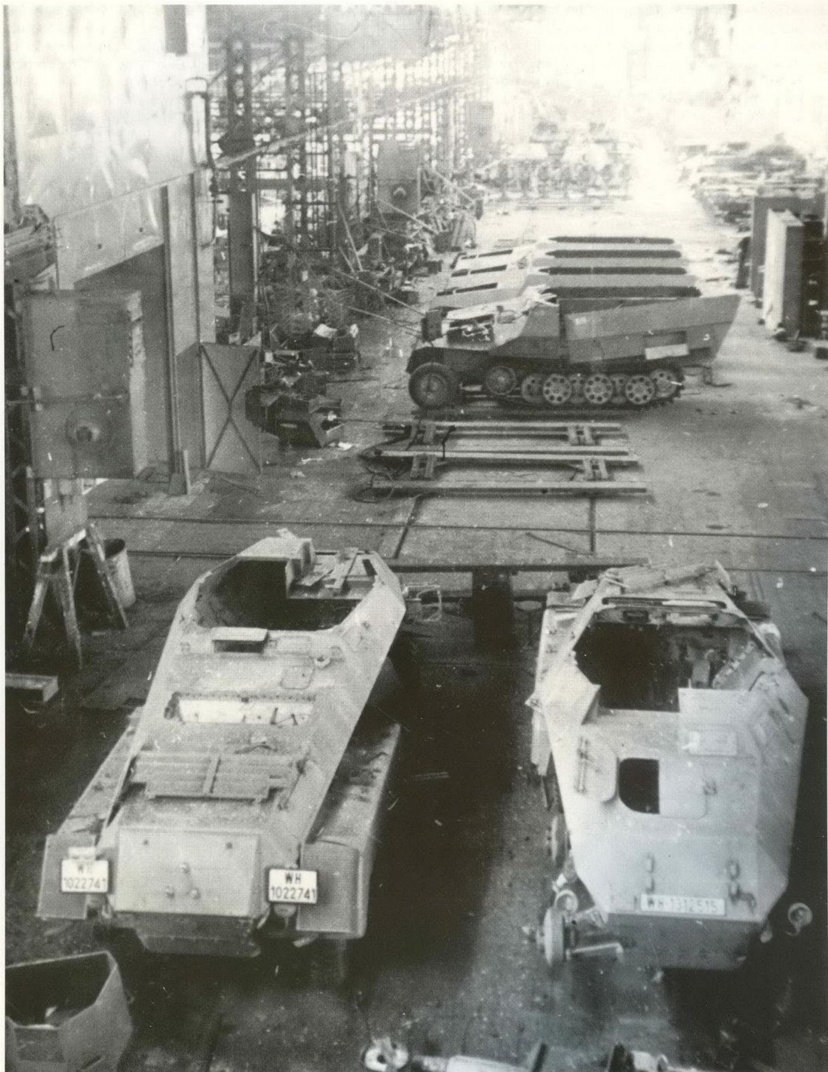
Zdobyte remontowane transportery Sd Kfz 251 i samochody pancerne Sd Kfz 233 (8x8) w zakładach naprawczych Schihau w Elblągu w lutym 1945 roku. The captured repaired Sd Kfz 251s APC and two Sd Kfz 233 (8x8) armored cars seen in Schihau repair plant in Elbing (now Elbląg in Poland), East Prussia, February 1945. [ASKM]
